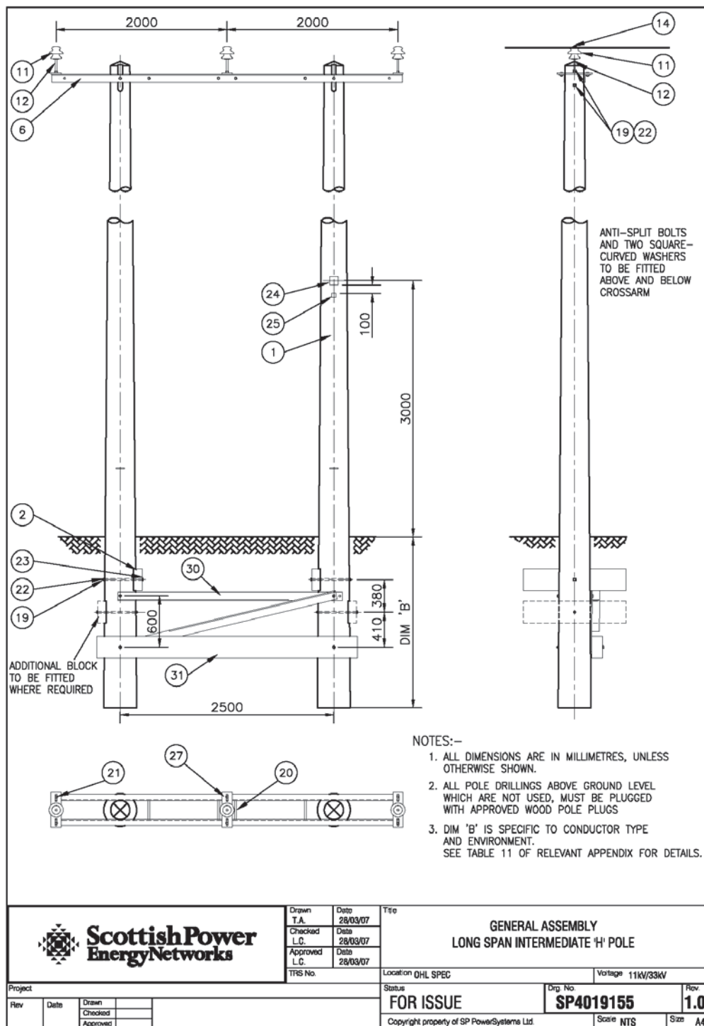
Figure 10 "H" Pole Intermediate Long Span (Drawing SP4019155)
